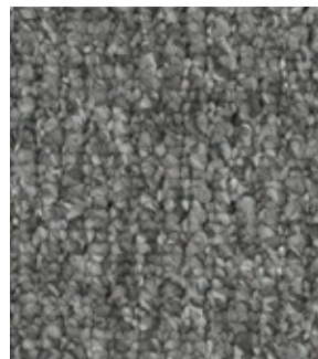
Phyllite 3806
